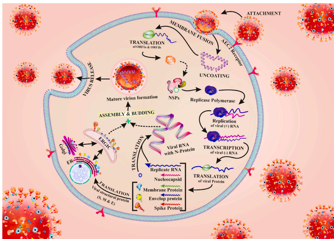
Fig. 2. The viral entry and replication of novel coronavirus pathogenesis.
